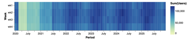
Fig. 4: An expert can produce a clean heatmap for Period \times Week \times sum(Users), but only by coordinating tightly coupled low-level parameters, including parsing, scale, mark width, and layout.
