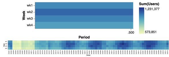
Fig. 3: A simple specification fails in two different ways: temporal interpretation misparses the period field, while nominal interpretation produces an overcrowded layout.
